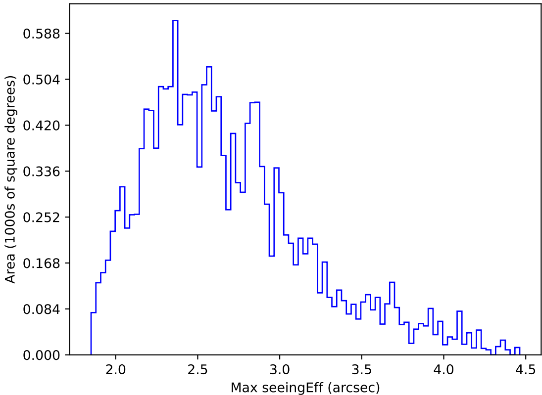
too_elab_r32_d3_ugrizy_v3.4_10yrs WFD r band: Max seeingEff
