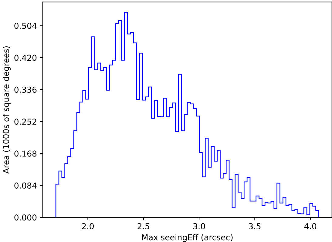
too_elab_r32_d3_ugrizy_v3.4_10yrs WFD g band: Max seeingEff
