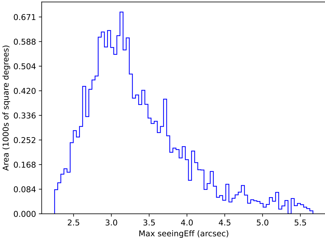
too_elab_r32_d3_ugrizy_v3.4_10yrs WFD all bands: Max seeingEff
