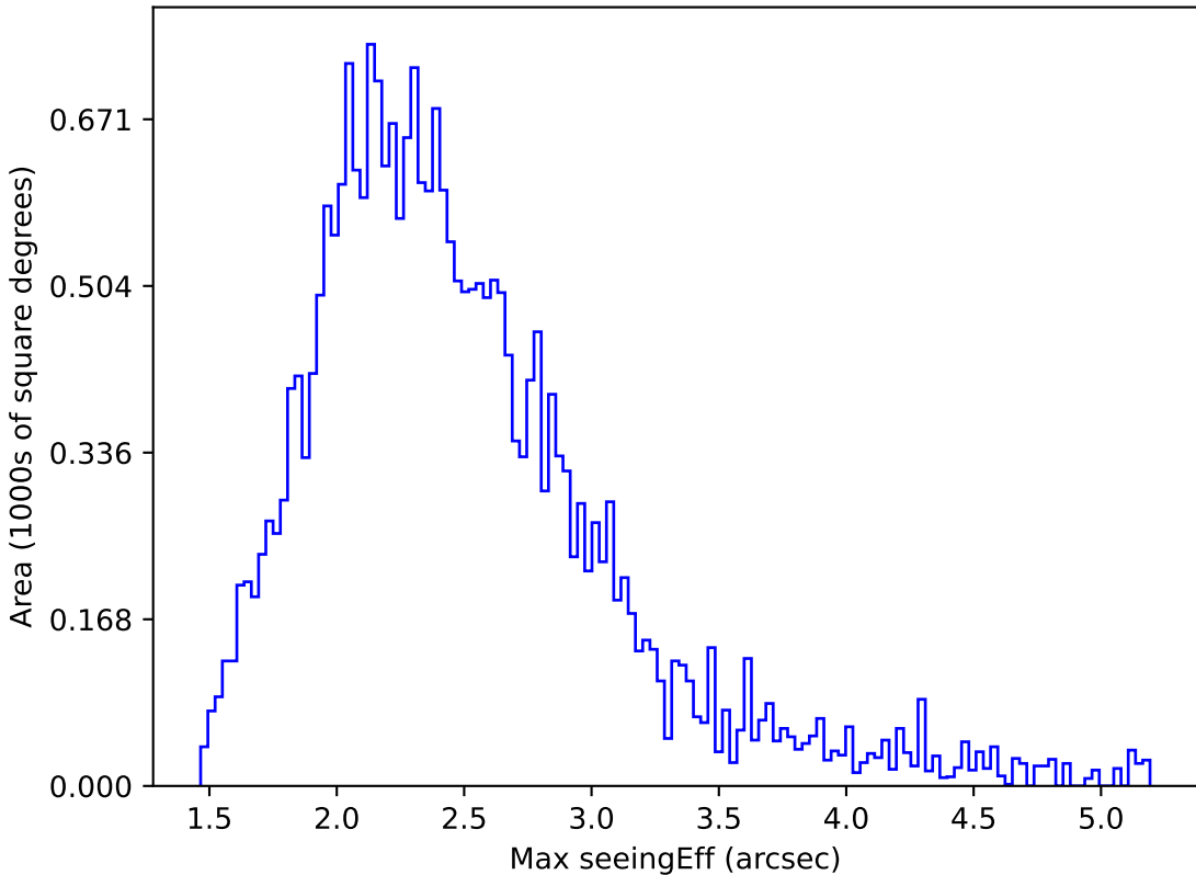
too_elab_r32_d3_ugrizy_v3.4_10yrs All sky z band: Max seeingEff
