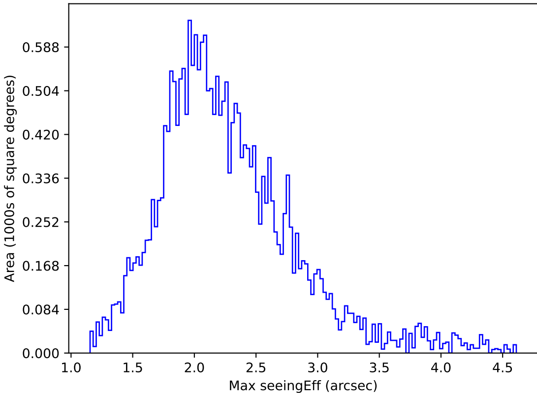
too_elab_r32_d3_ugrizy_v3.4_10yrs All sky y band: Max seeingEff
