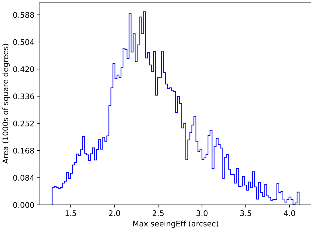
too_elab_r32_d3_uigrizy_v3.4_10yrs All sky u band: Max seeingEff
