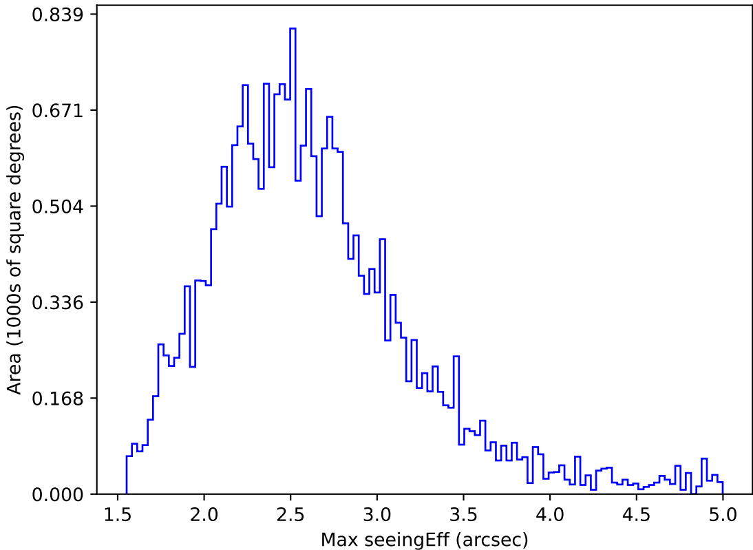
too_elab_r32_d3_ugrizy_v3.4_10yrs All sky i band: Max seeingEff
