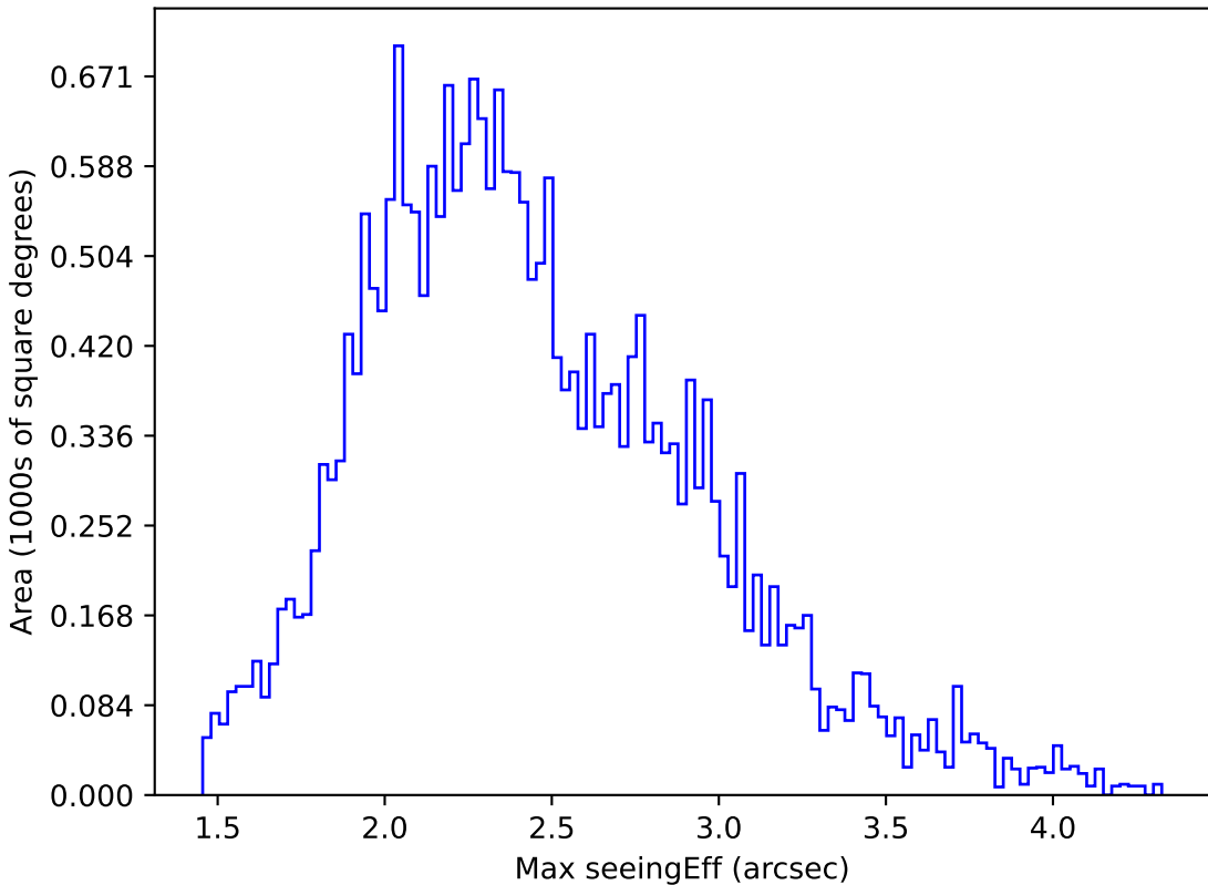
too_elab_r32_d3_ugrizy_v3.4_10yrs All sky g band: Max seeingEff
