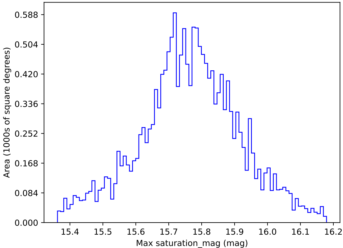
too_elab_r32_d3_ugrizy_v3.4_10yrs WFD r band: Max saturation_mag
