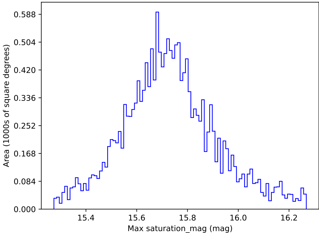
too_elab_r32_d3_ugrizy_v3.4_10yrs WFD g band: Max saturation_mag
