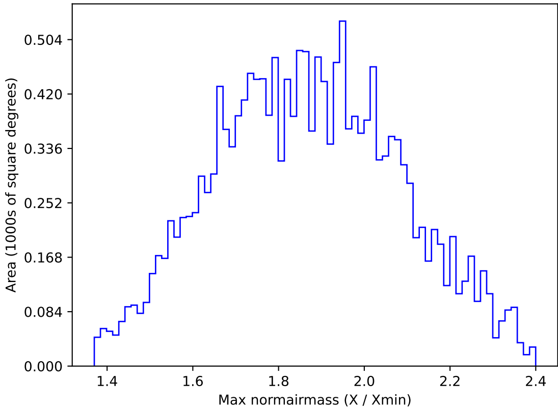
too_elab_r32_d3_ugrizy_v3.4_10yrs WFD g band: Max normairmass
