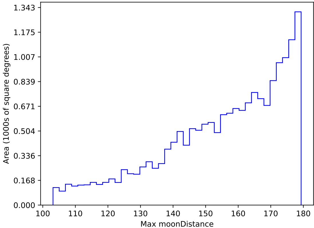
too_elab_r32_d3_ugrizy_v3.4_10yrs WFD i band: Max moonDistance
