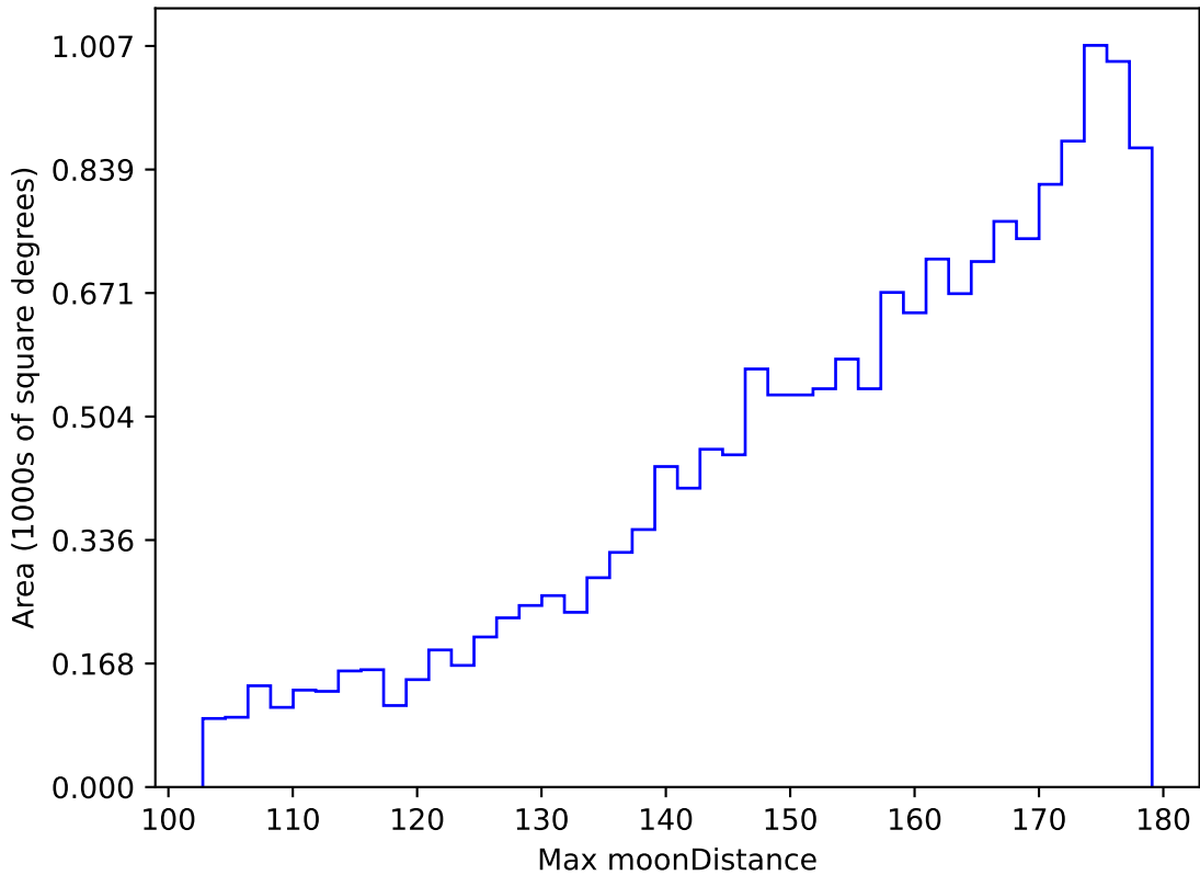
too_elab_r32_d3_ugrizy_v3.4_10yrs WFD g band: Max moonDistance
