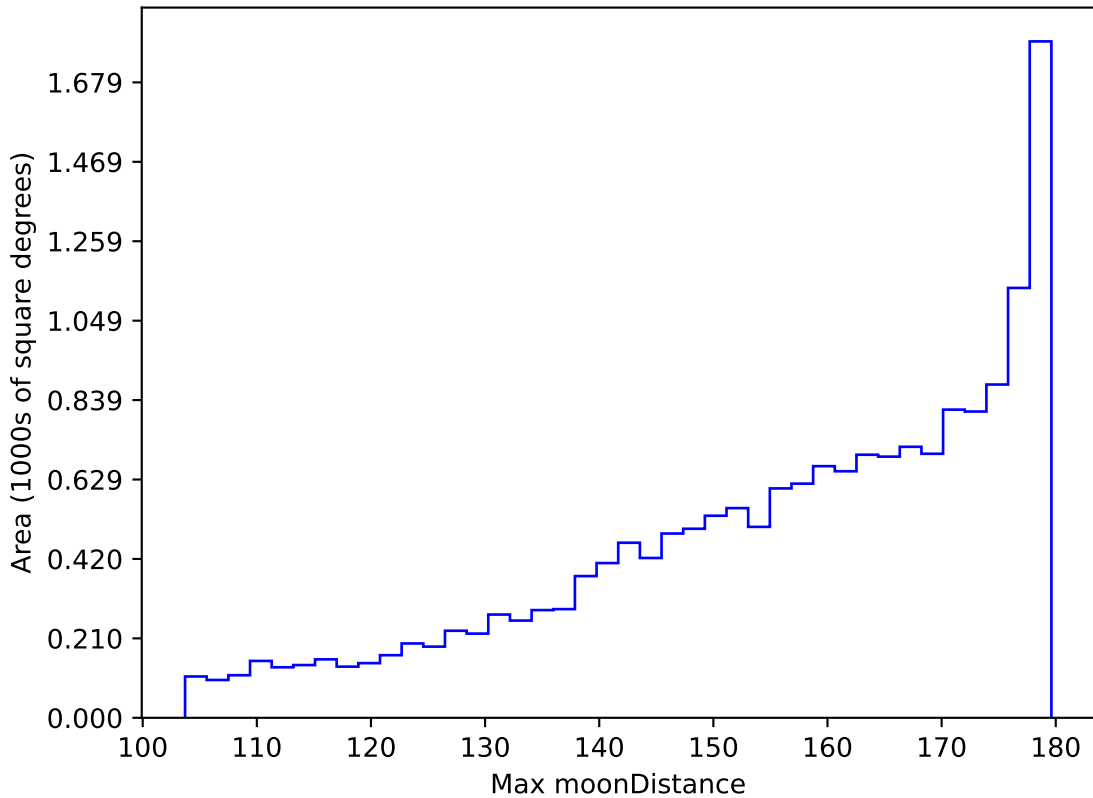
too_elab_r32_d3_ugrizy_v3.4_10yrs WFD all bands: Max moonDistance
