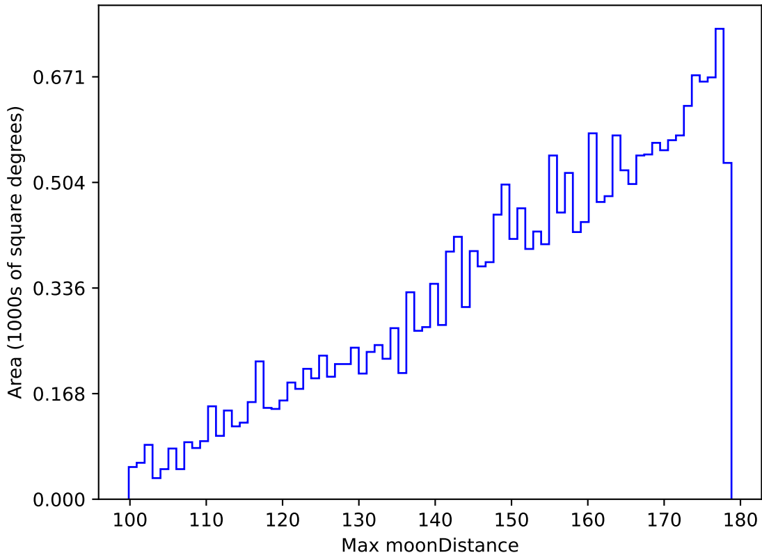
too_elab_r32_d3_ugrizy_v3.4_10yrs All sky u band: Max moonDistance
