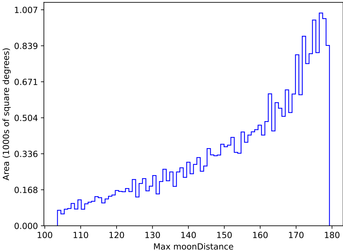
too_elab_r32_d3_ugrizy_v3.4_10yrs All sky i band: Max moonDistance
