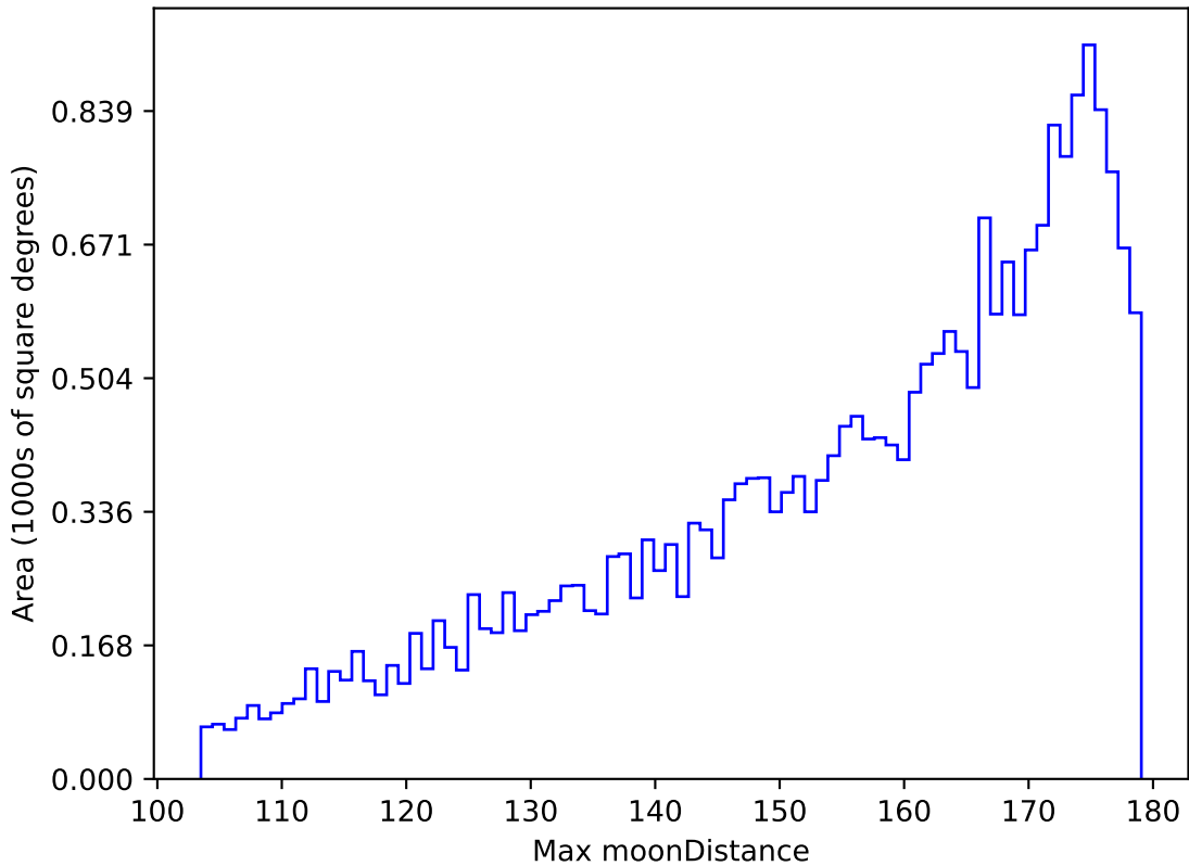
too_elab_r32_d3_ugrizy_v3.4_10yrs All sky g band: Max moonDistance
