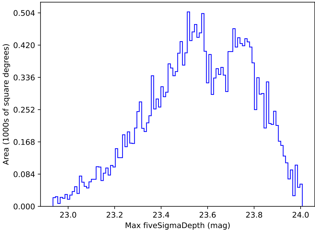
too_elab_r32_d3_ugrizy_v3.4_10yrs Yr 1 u band: Max fiveSigmaDepth
