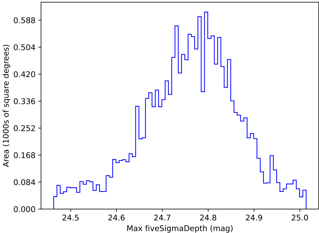
too_elab_r32_d3_ugrizy_v3.4_10yrs WFD r band: Max fiveSigmaDepth
