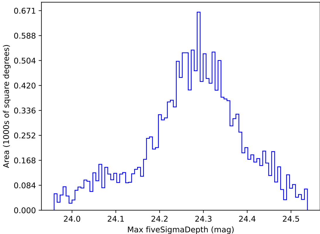
too_elab_r32_d3_ugrizy_v3.4_10yrs WFD i band: Max fiveSigmaDepth
