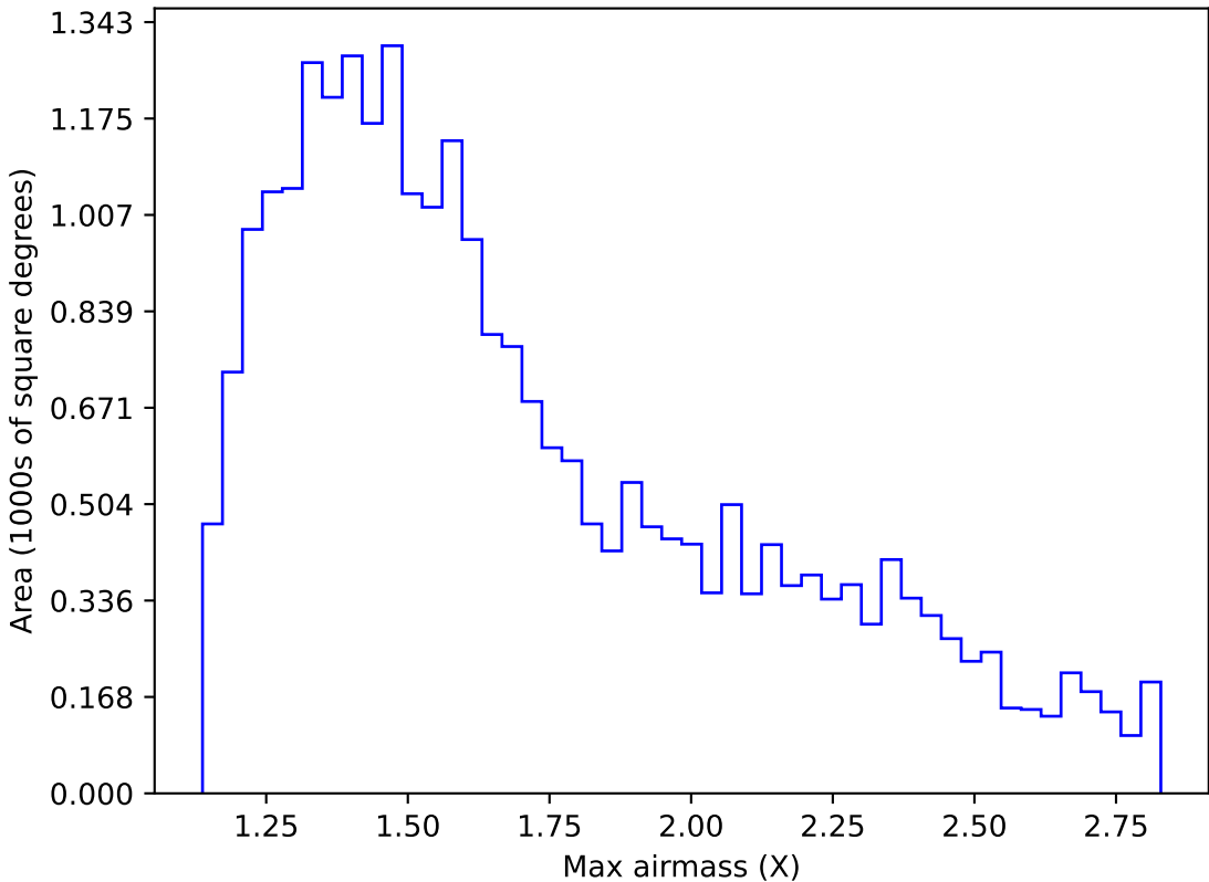
too_elab_r32_d3_ugrizy_v3.4_10yrs Yr 1 z band: Max airmass
