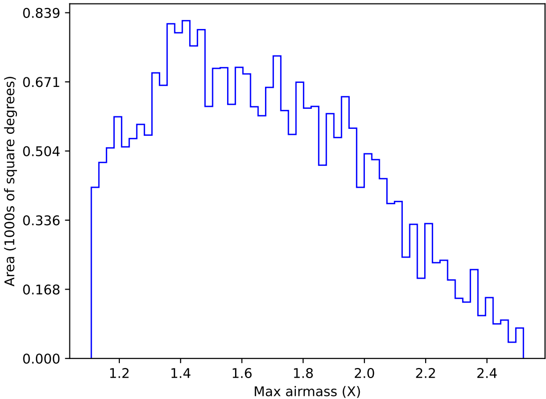
too_elab_r32_d3_ugrizy_v3.4_10yrs Yr 1 g band: Max airmass
