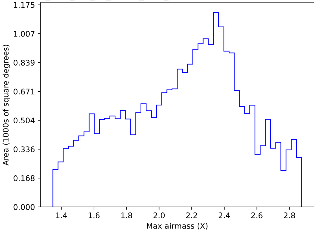
too_elab_r32_d3_ugrizy_v3.4_10yrs Yr 1 all bands: Max airmass
