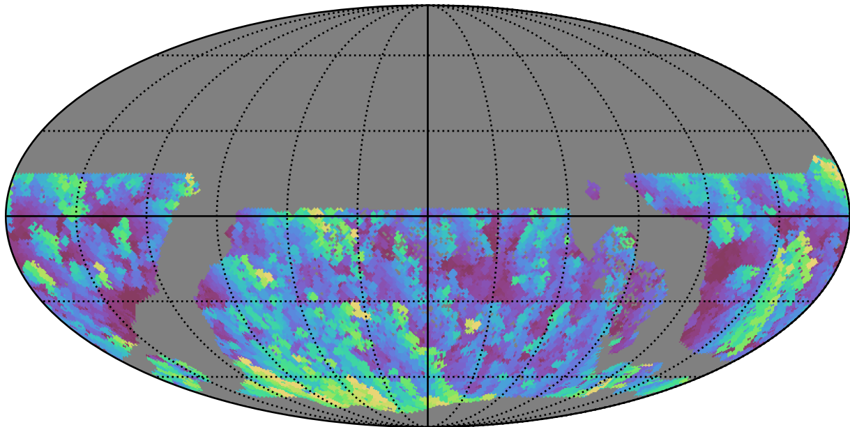
too_elab_r32_d3_ugrizy_v3.4_10yrs WFD u band: Max airmass
