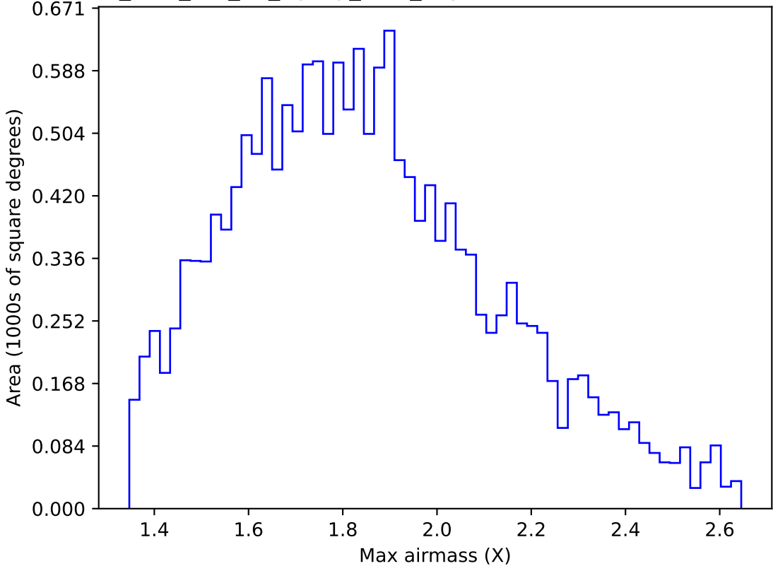
too_elab_r32_d3_ugrizy_v3.4_10yrs WFD u band: Max airmass
