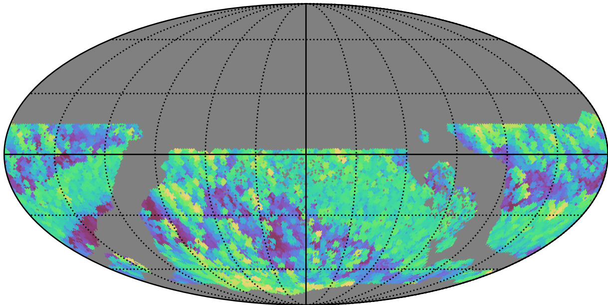
too_elab_r32_d3_ugrizy_v3.4_10yrs WFD r band: Max airmass
