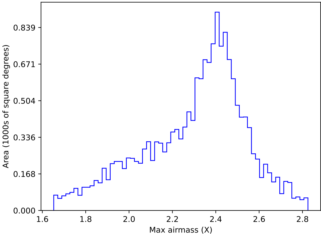
too_elab_r32_d3_ugrizy_v3.4_10yrs WFD r band: Max airmass
