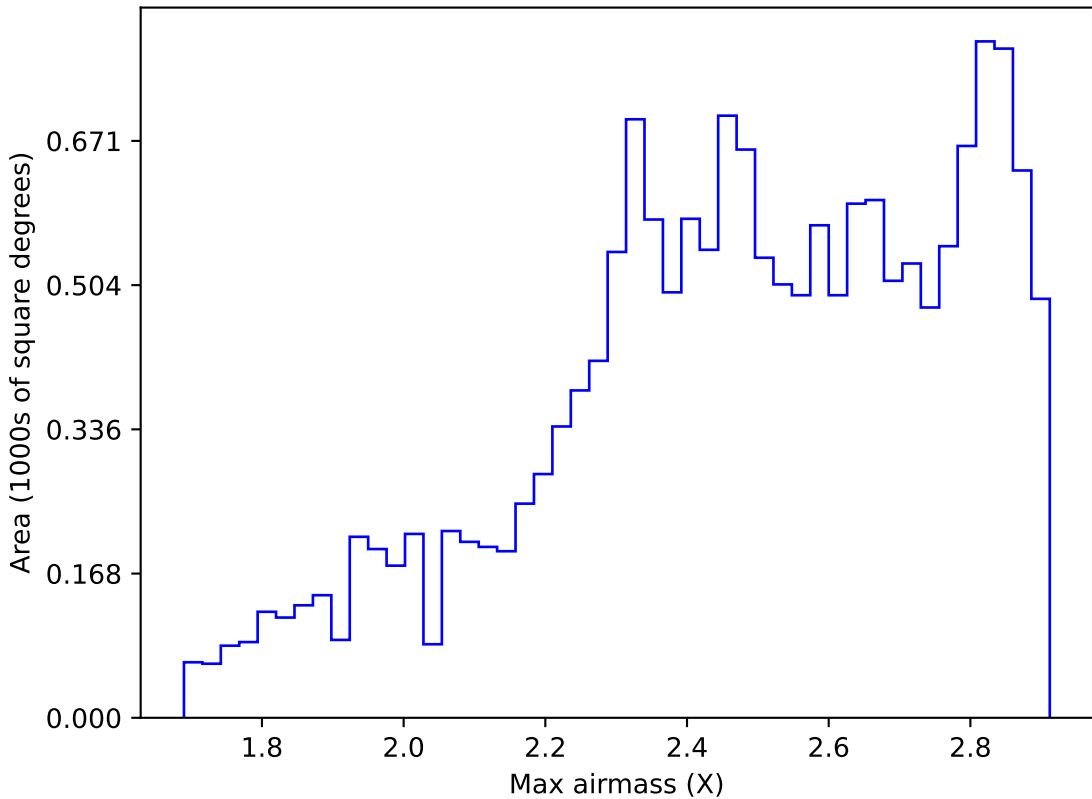
too_elab_r32_d3_ugrizy_v3.4_10yrs WFD i band: Max airmass
