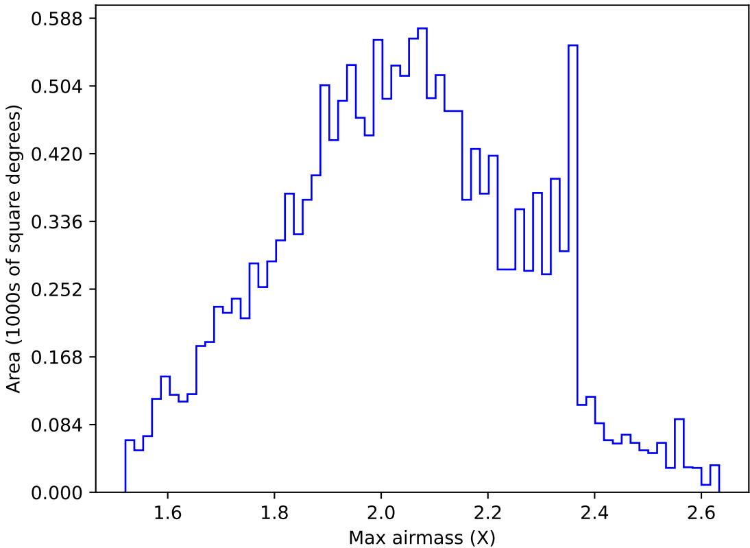
too_elab_r32_d3_ugrizy_v3.4_10yrs WFD g band: Max airmass
