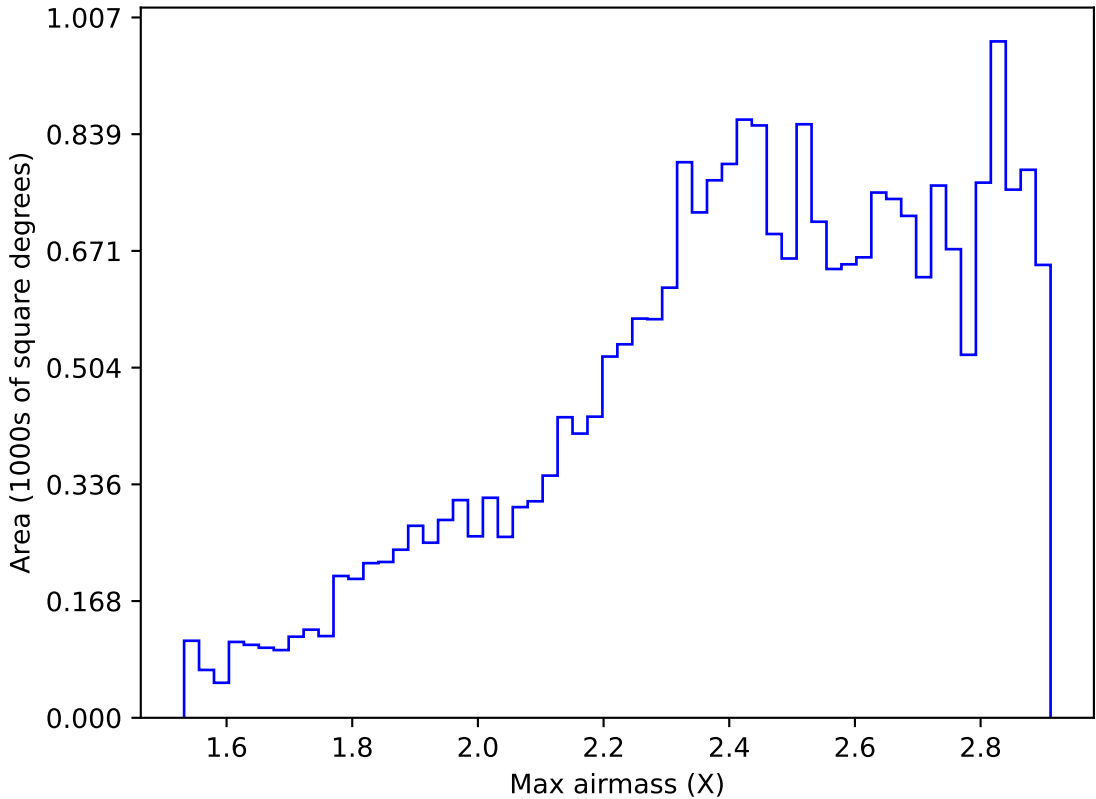
too_elab_r32_d3_ugrizy_v3.4_10yrs All sky z band: Max airmass
