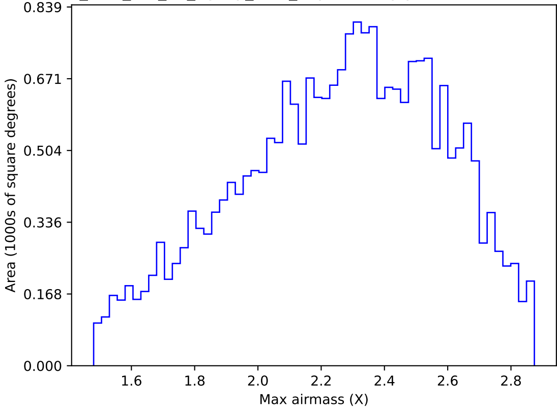
too_elab_r32_d3_ugrizy_v3.4_10yrs All sky y band: Max airmass
