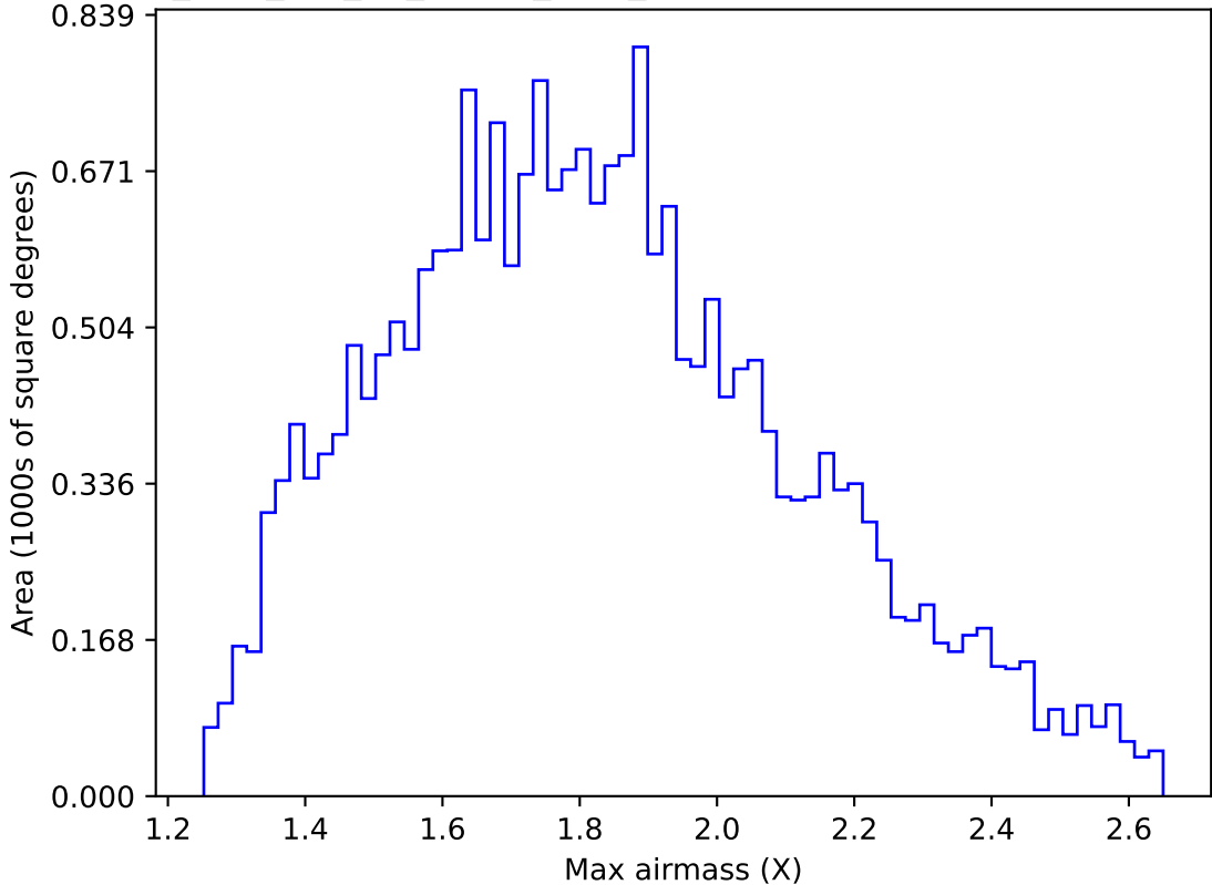
too_elab_r32_d3_ugrizy_v3.4_10yrs All sky u band: Max airmass
