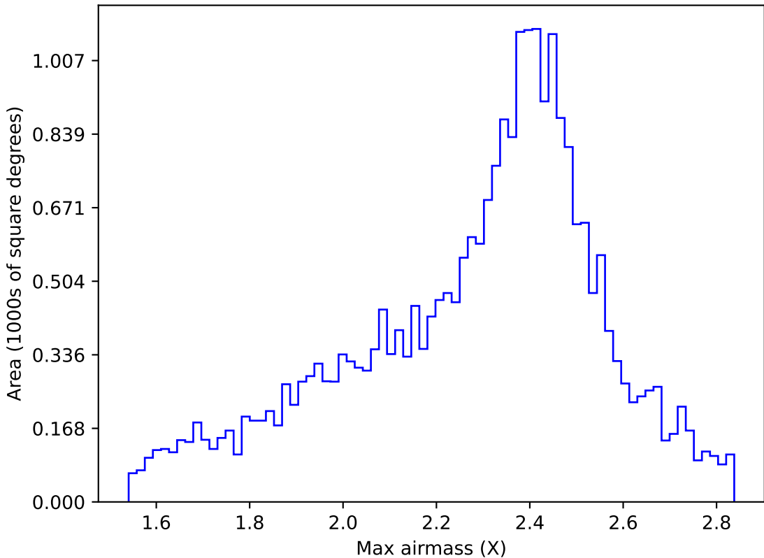
too_elab_r32_d3_ugrizy_v3.4_10yrs All sky r band: Max airmass
