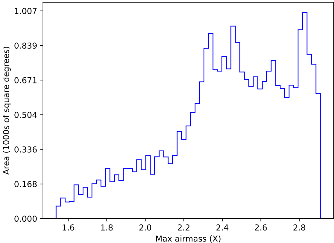
too_elab_r32_d3_ugrizy_v3.4_10yrs All sky i band: Max airmass
