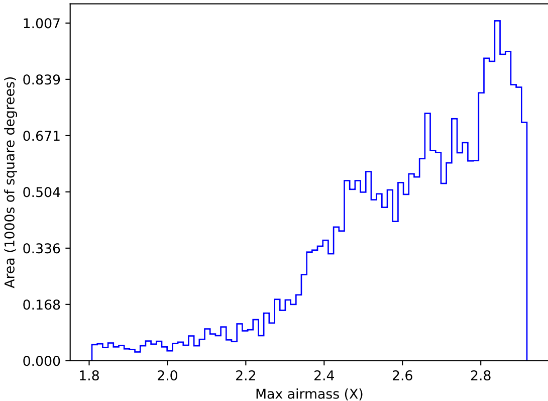
too_elab_r32_d3_ugrizy_v3.4_10yrs All sky all bands: Max airmass
