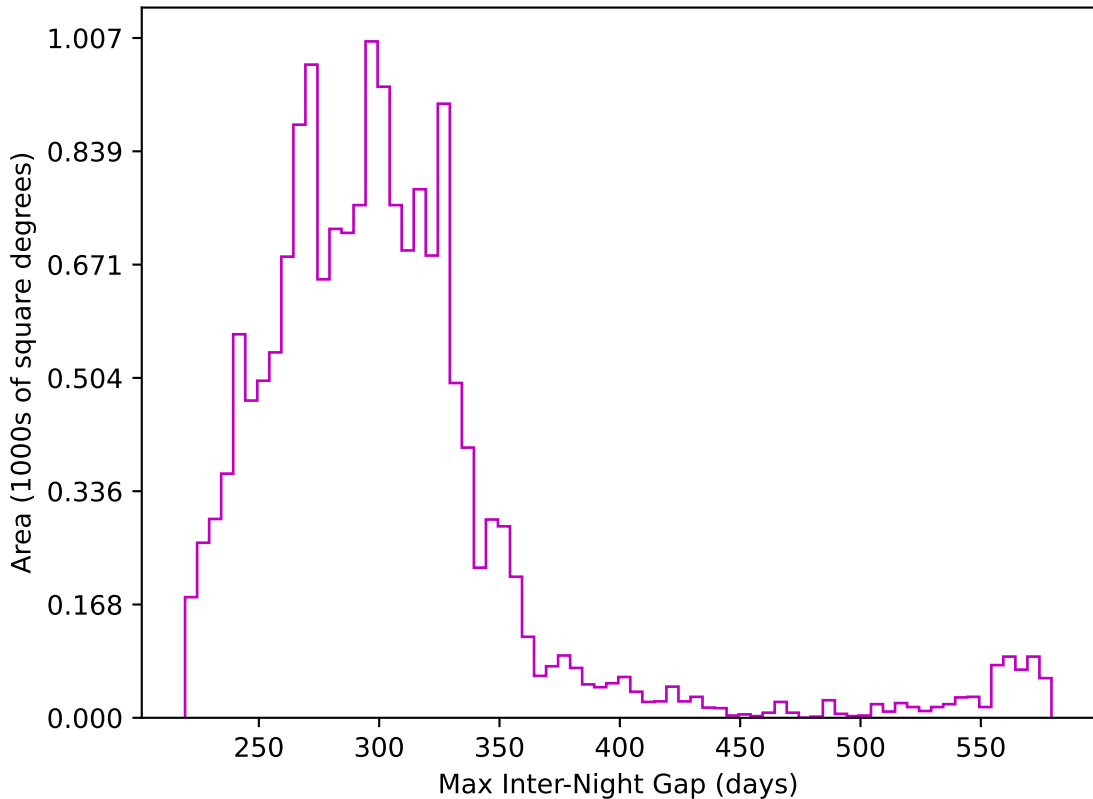
too_elab_r32_d3_ugrizyv3.4_10yrs WFD z band: Max Inter-Night Gap
