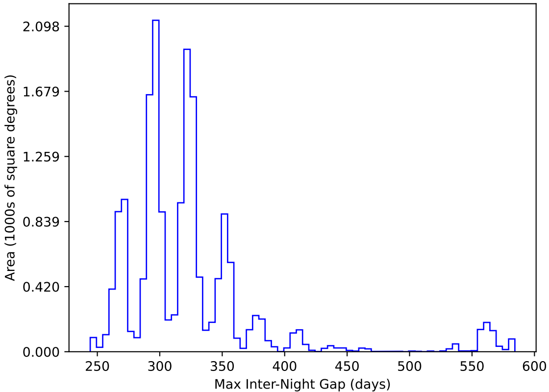
too_elab_r32_d3_ugrizy_v3.4_10yrs WFD y band: Max Inter-Night Gap
