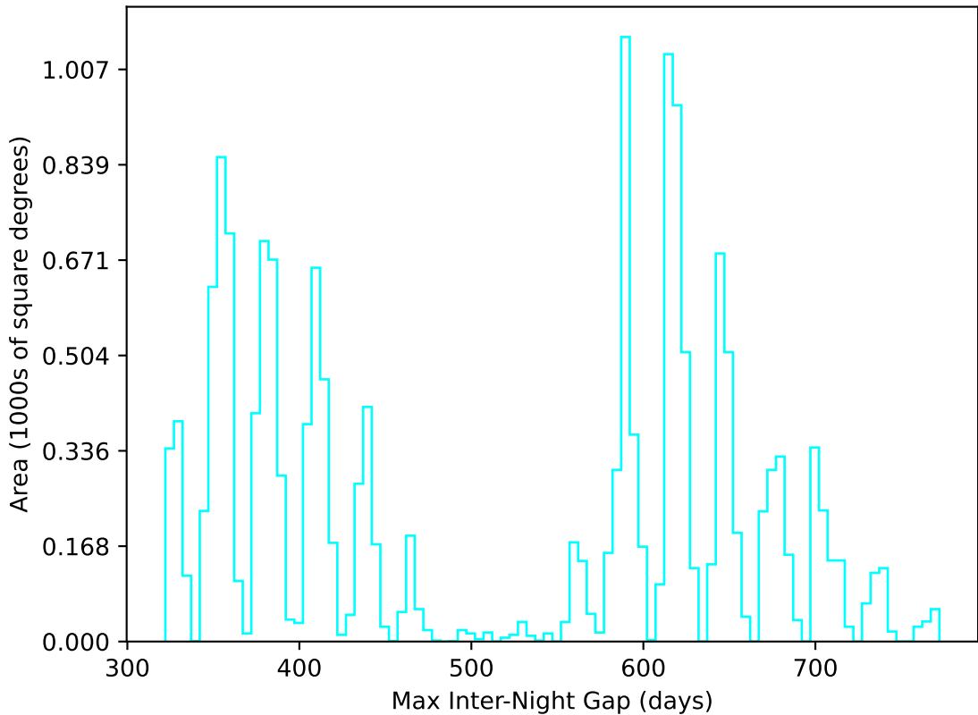
too_elab_r32_d3_ugrizy_v3.4_10yrs WFD u band: Max Inter-Night Gap
