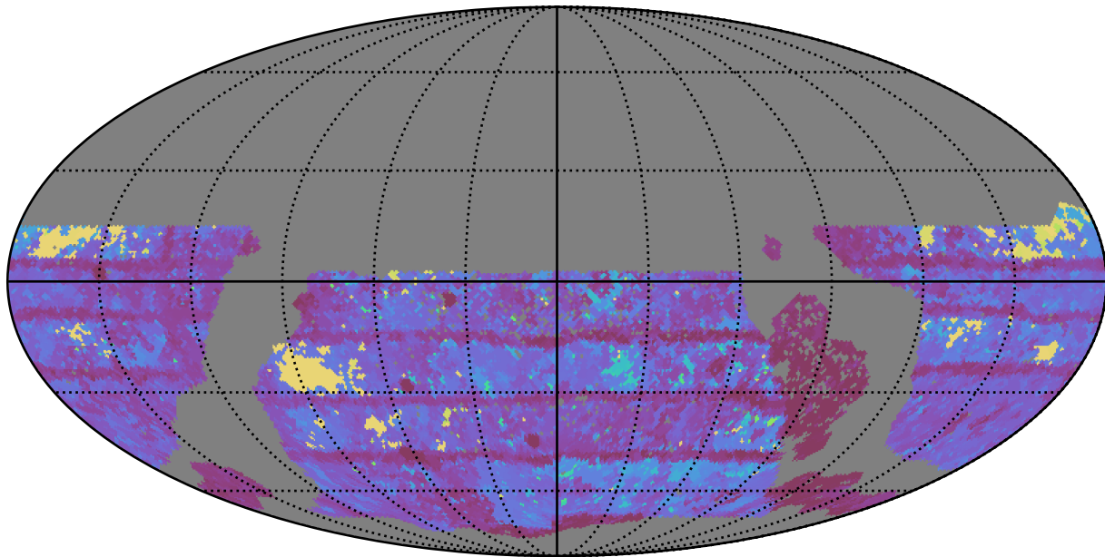
too_elab_r32_d3_ugrizy_v3.4_10yrs WFD r band: Max Inter-Night Gap
