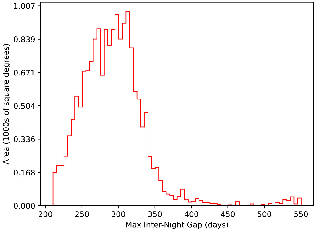
too_elab_r32_d3_ugrizy_v3.4_10yrs WFD i band: Max Inter-Night Gap
