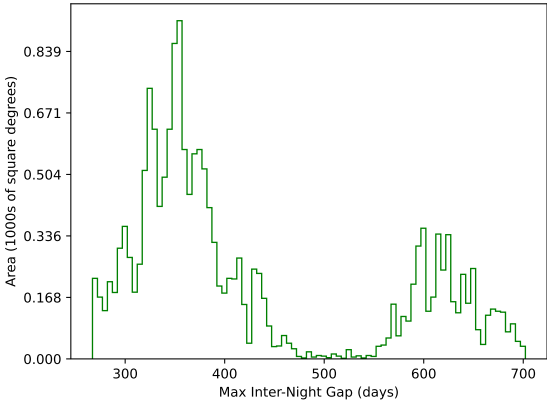
too_elab_r32_d3_ugrizy_v3.4_10yrs WFD g band: Max Inter-Night Gap
