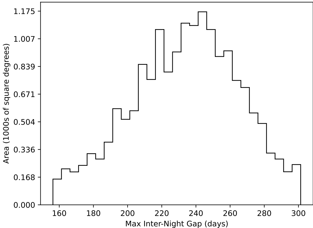
too_elab_r32_d3_ugrizy_v3.4_10yrs WFD all bands: Max Inter-Night Gap
