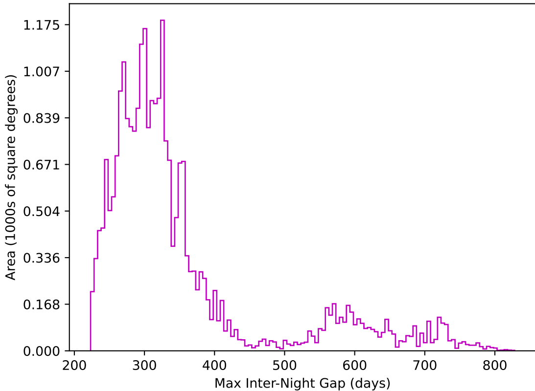
too_elab_r32_d3_ugrizy_v3.4_10yrs All sky z band: Max Inter-Night Gap
