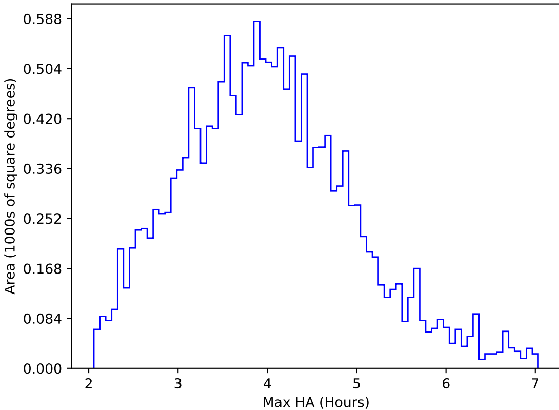
too_elab_r32_d3_ugrizy_v3.4_10yrs WFD u band: Max HA
