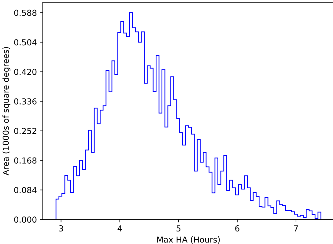
too_elab_r32_d3_ugrizy_v3.4_10yrs WFD r band: Max HA
