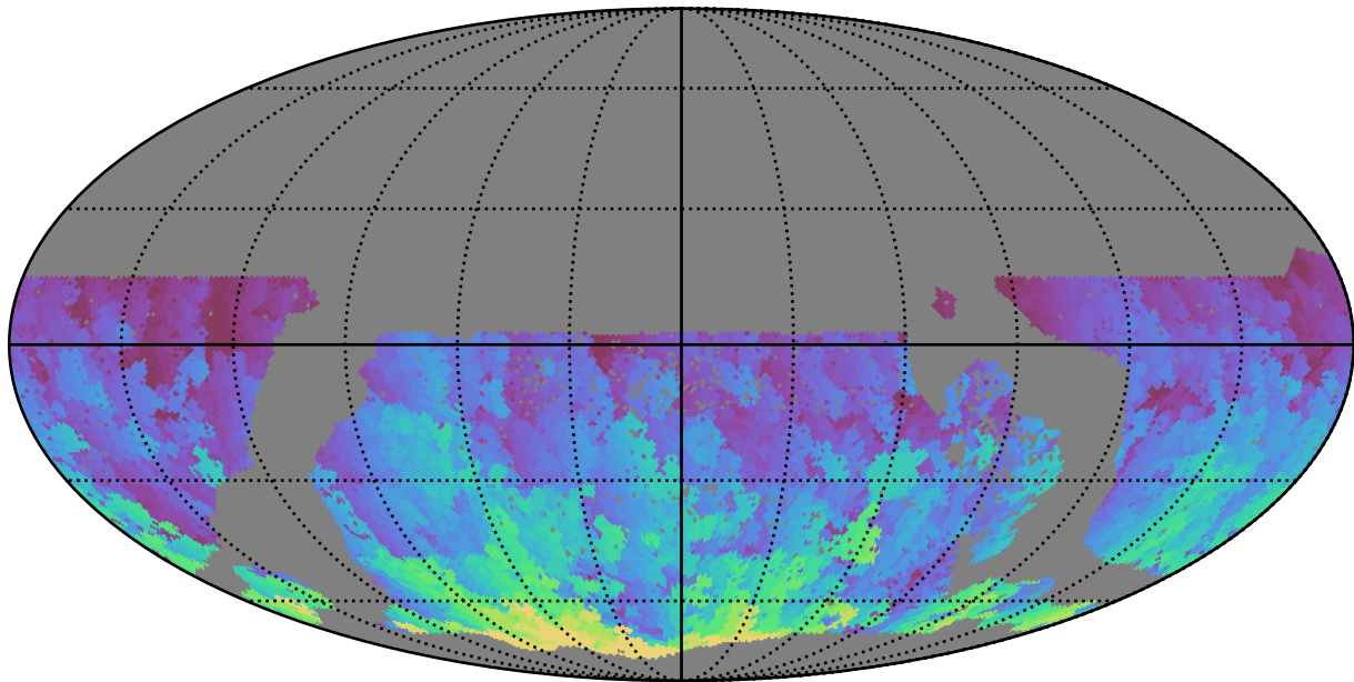
too_elab_r32_d3_ugrizy_v3.4_10yrs WFD g band: Max HA
