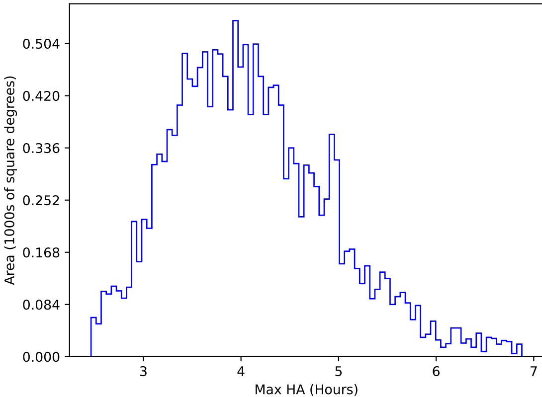
too_elab_r32_d3_ugrizy_v3.4_10yrs WFD g band: Max HA
