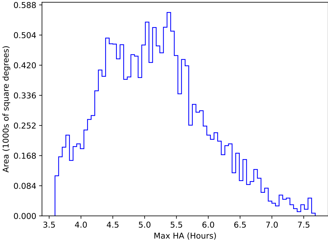
too_elab_r32_d3_ugrizy_v3.4_10yrs WFD all bands: Max HA
