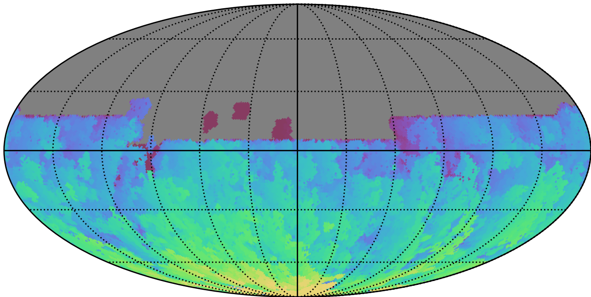
too_elab_r32_d3_ugrizy_v3.4_10yrs All sky u band: Max HA
