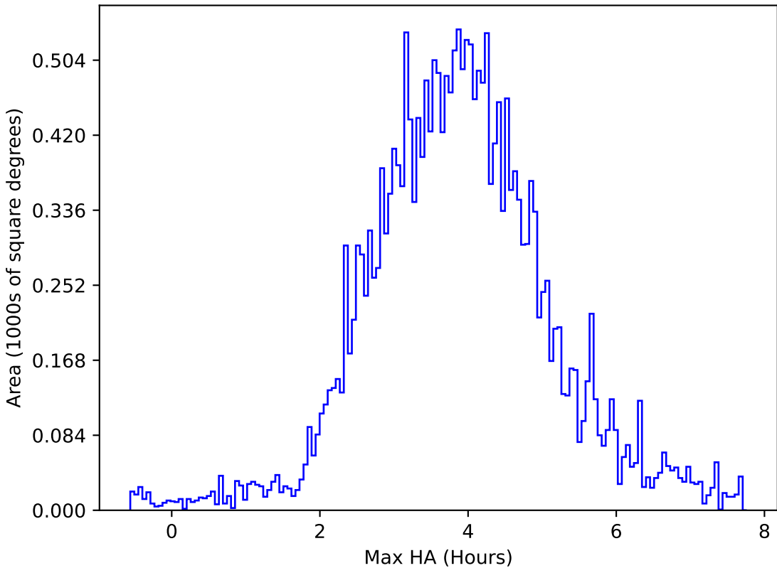
too_elab_r32_d3_ugrizy_v3.4_10yrs All sky u band: Max HA
